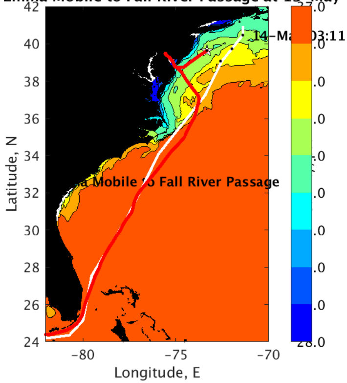
Salinity for Emma Mobile to Fall River Passage at 13-May-2022 00:00:00
